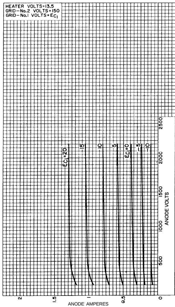
Figure 6 - Typical Anode Characteristics 92CM-11289
