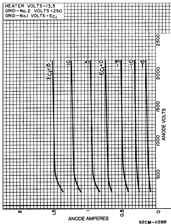
Figure 4 - Typical Anode Characteristics
