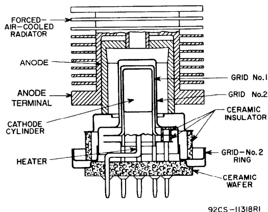
Figure 1 - Structural Arrangement
