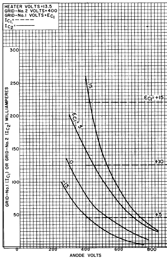
Figure 3 - Typical Characteristics
