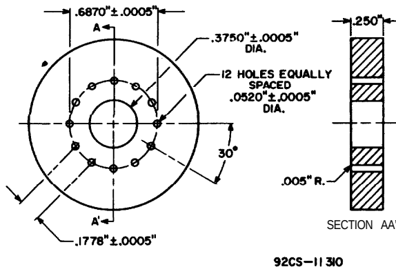
Figure 12 - Gauge Drawing JEDEC No.GE11-1
