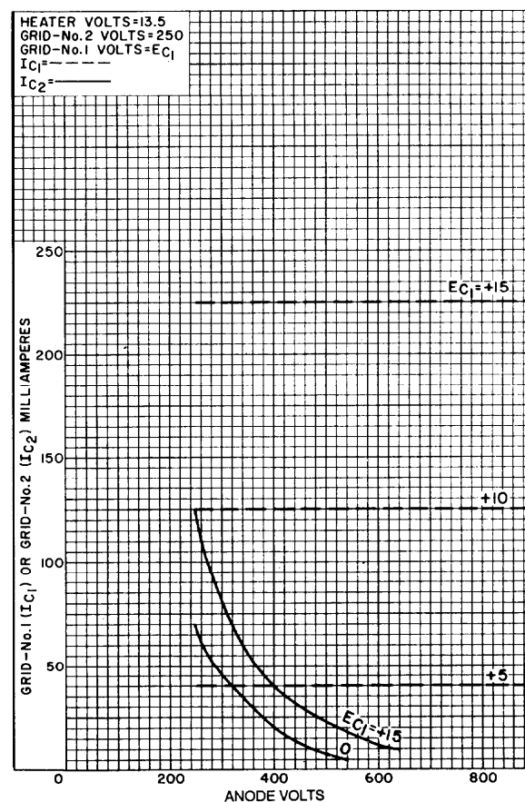
Figure 5 - Typical Characteristics
